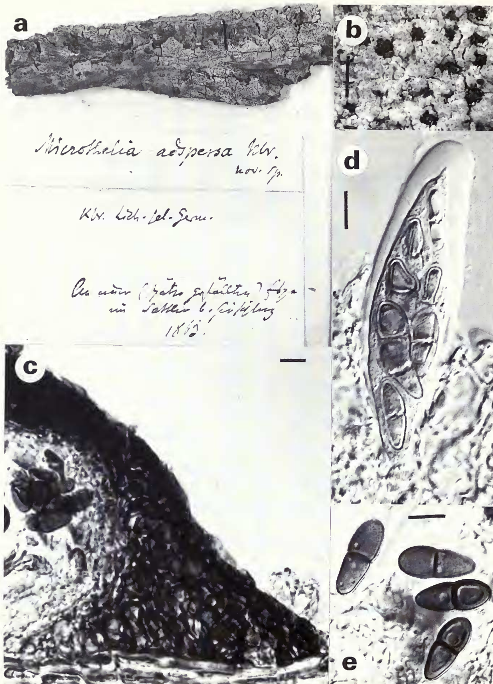
Fig. 4 ' Microthelia ' adpersa Körber (WRSL) (a) General view of packet; (b) Surface view of ascomata; scale = 500 µm; (c) Detail of exciple: textura angularis ; (d) Ascus and ascospores; (e) Ascospores; scale = 10 µm.
